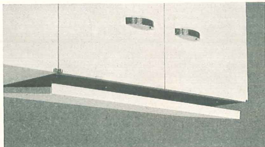
BOTTOM PLATE—Recommended on under side of 18" high wall cabinets used over refrigerator or range. Also finishes bottoms of 30" high cabinets smoothly.
